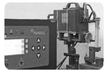
INDUCTION BRAZING
